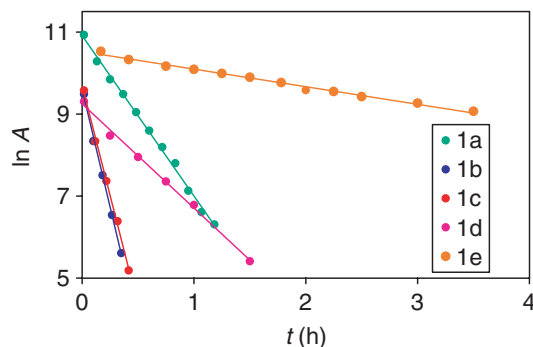
Figure 2 Plots of values of \ln A vs time for acidolysis of \alpha , \alpha -dialkyl glycine derivatives 1a–1e .
