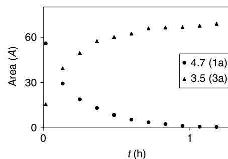
Figure 1 Plot of peak areas, A, vs time for an acidolysis experiment with compound 1a . The figures in the box are the observed HPLC retention times (min).
